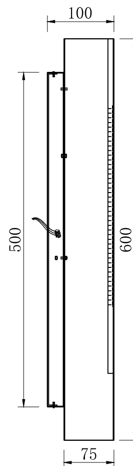
Side view
